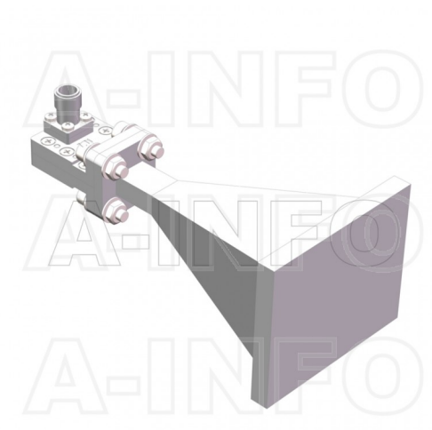
LB-28-20-64-C-2.4FSPO Frequency Extended Standard Gain Horn Antenna 22.5-45GHz 20dB Gain 2.4mm Female
