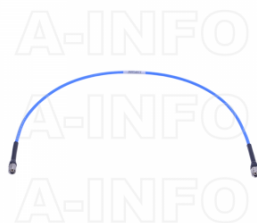
2.4M-2.4M-B020-500 Flexible Cable Assembly 500mm DC-50GHz 2.4mm Male to 2.4mm Male
